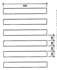
PEDESTRIAN CROSSING 1:50
