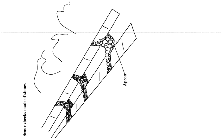
FIGURE C.7 SCOUR CHECKS
